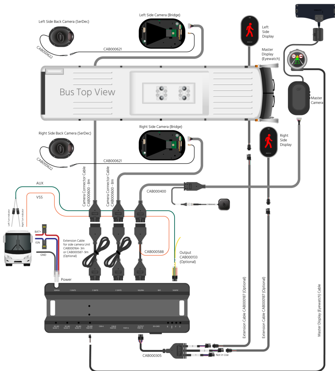
Connection scheme with Mobileye 8 unit including 4G modem.
