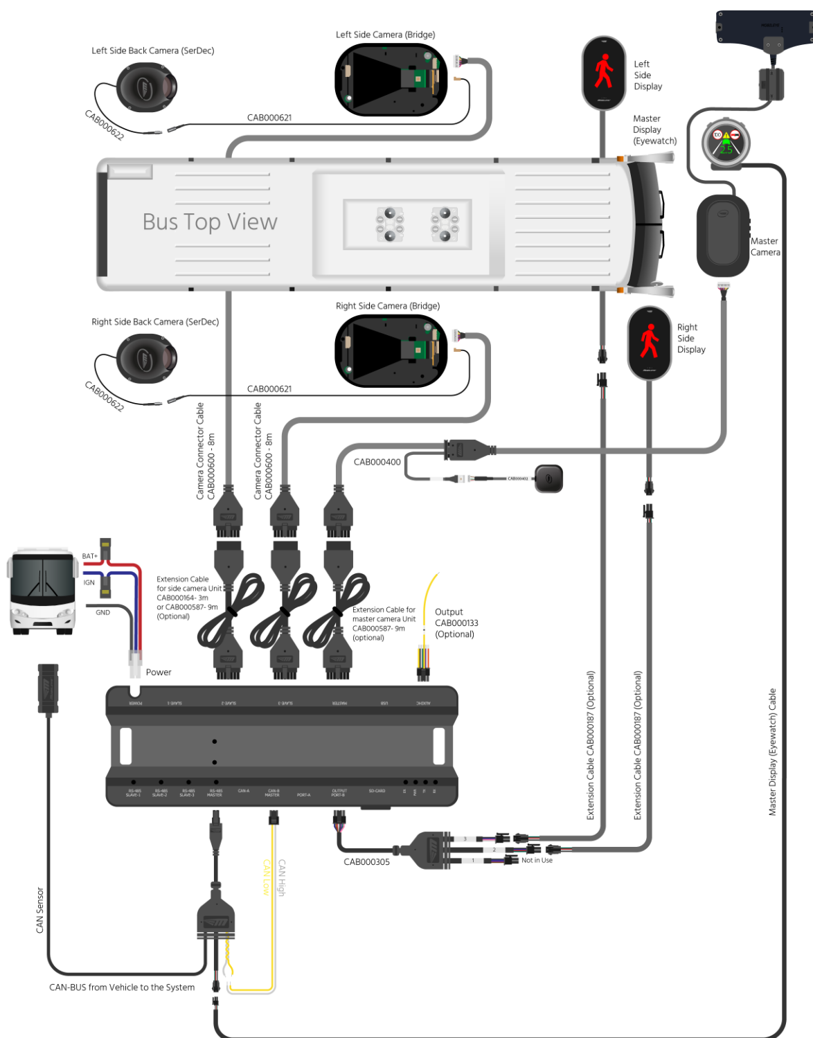
Connection scheme with Mobileye 8 unit including 4G modem.
