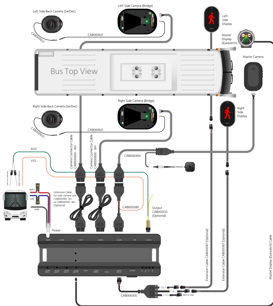
Connection scheme with Mobileye 8 unit including 3G modem.
