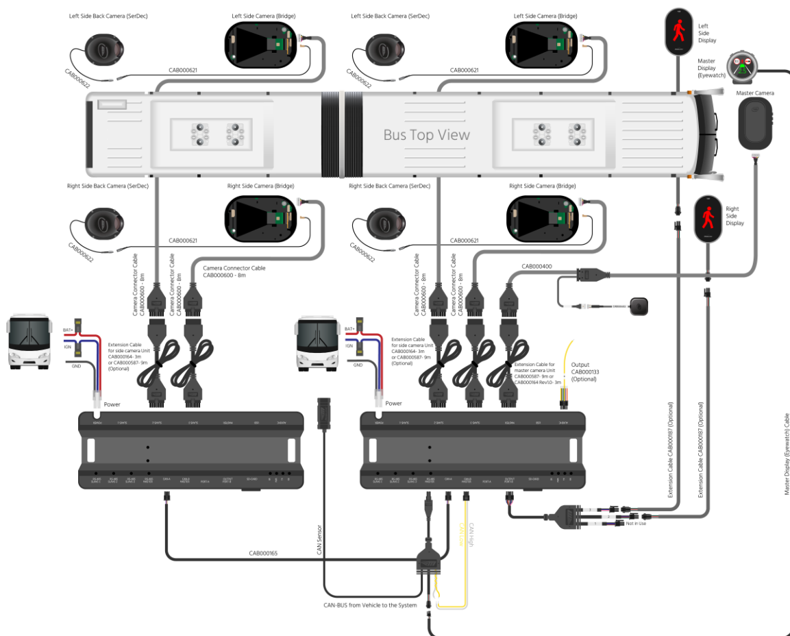
Connection scheme with Mobileye 8 unit including 3G modem.
